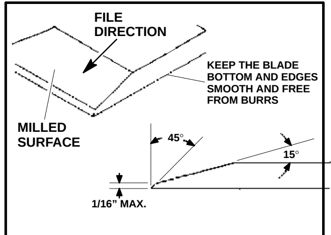
Figure 49 Blade Sharpening (Bottom Blade)
