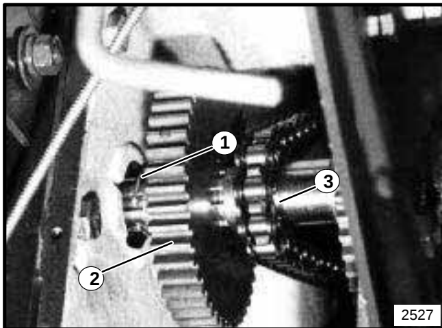
FIGURE 38 1. Snap Ring 2. Gear 3. Master Link
