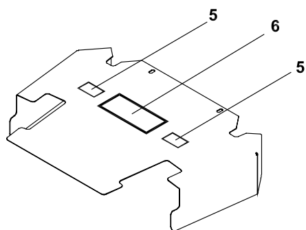
FLOATING DECKS
