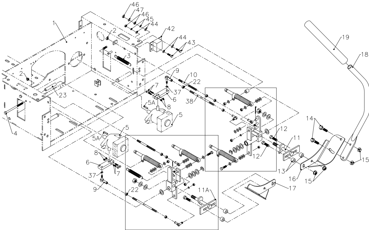
Power Box (front) Drive Parts Figure 8A Serial No. 2188 & Up
