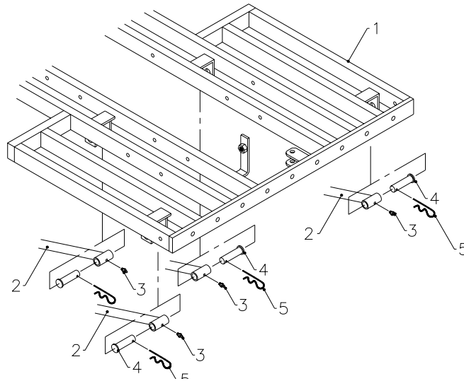
Mower Frame & Belts Figure 18
