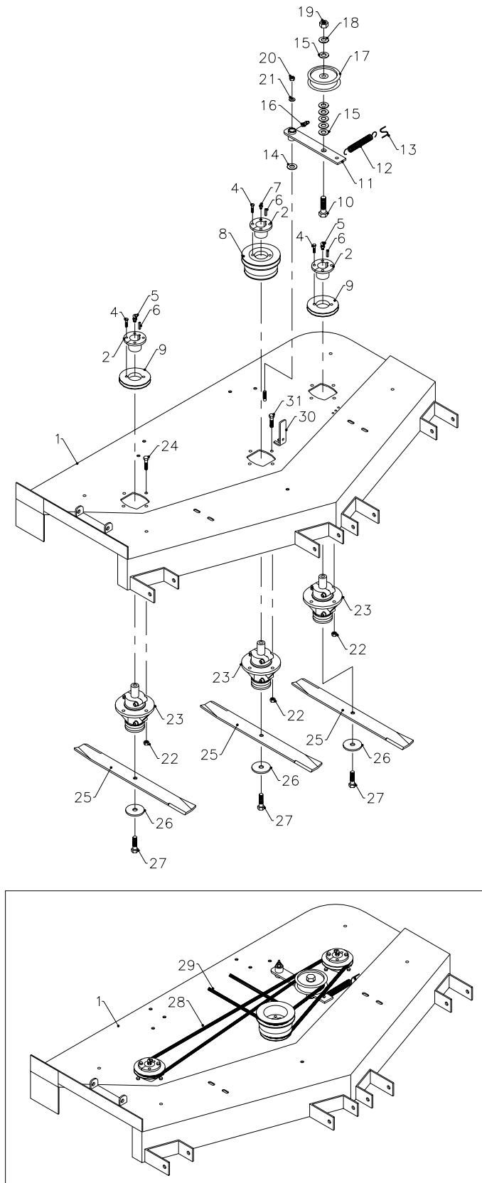
Drive Parts & Belts Figure 16
