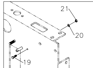
Figure 1A Frame with Kohler Engine
