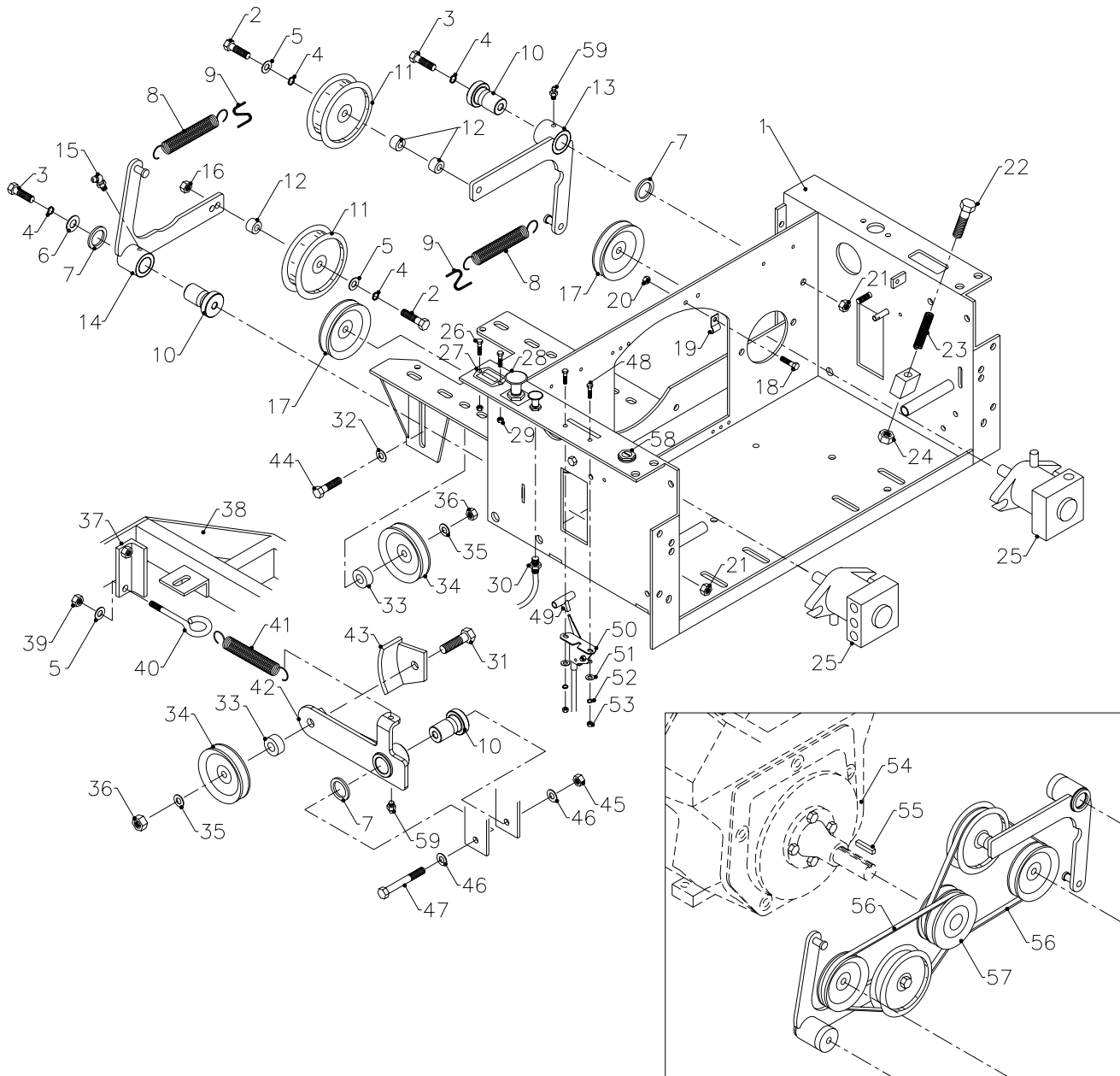
Power Box (rear) Drive Parts Figure 9
