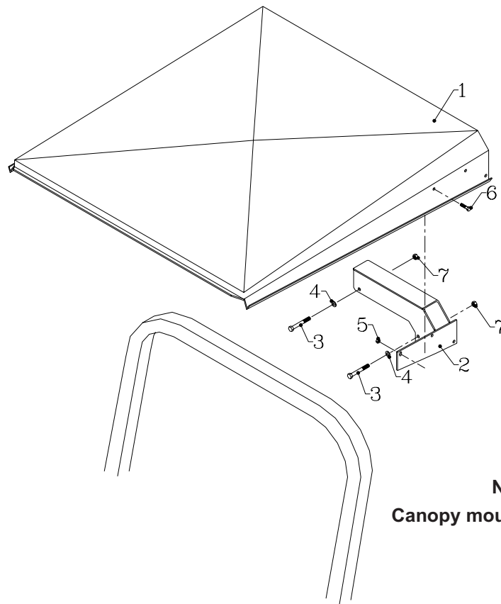
SH325 Sun Shade Canopy Figure 8-2
