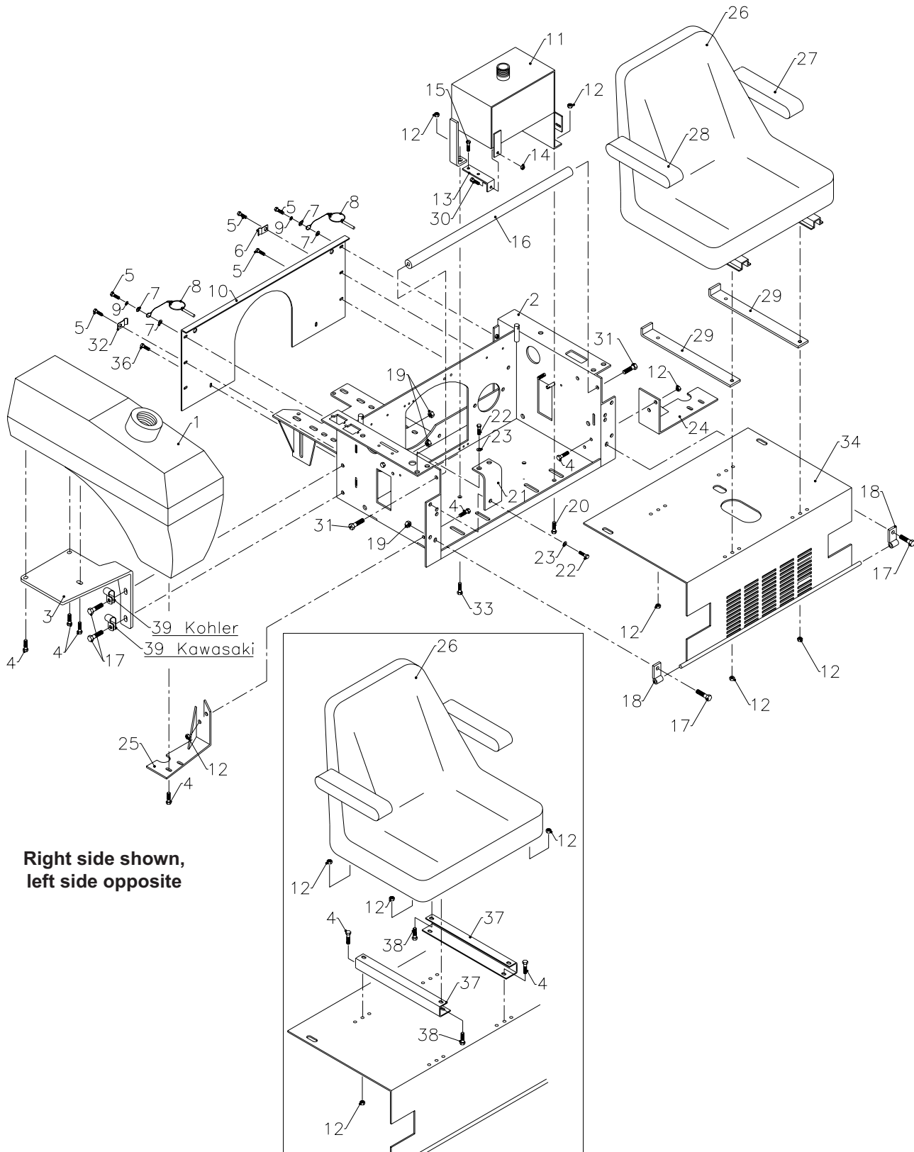
Upper Frame Parts Figure 1
