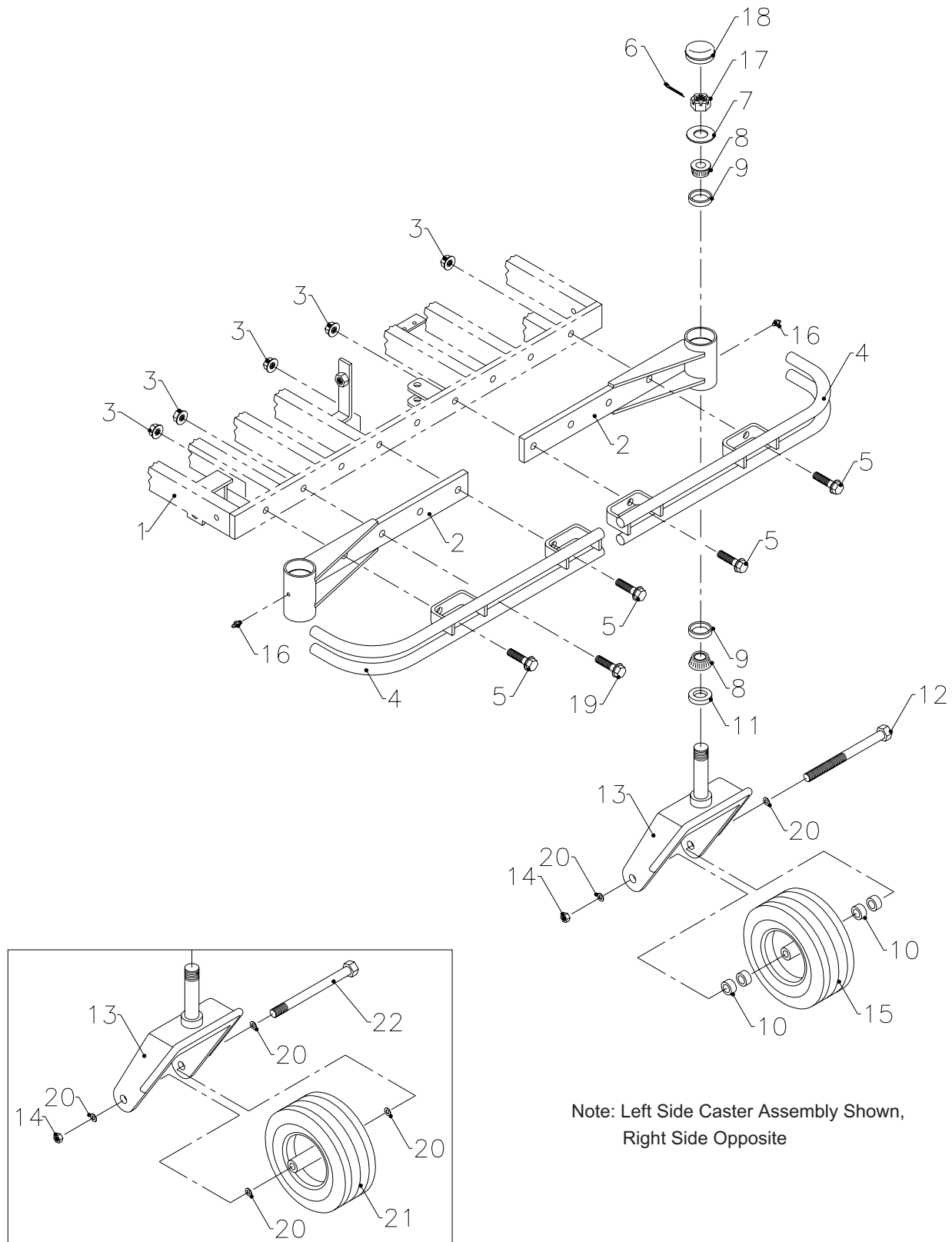
Front Bumper Figure 2a
