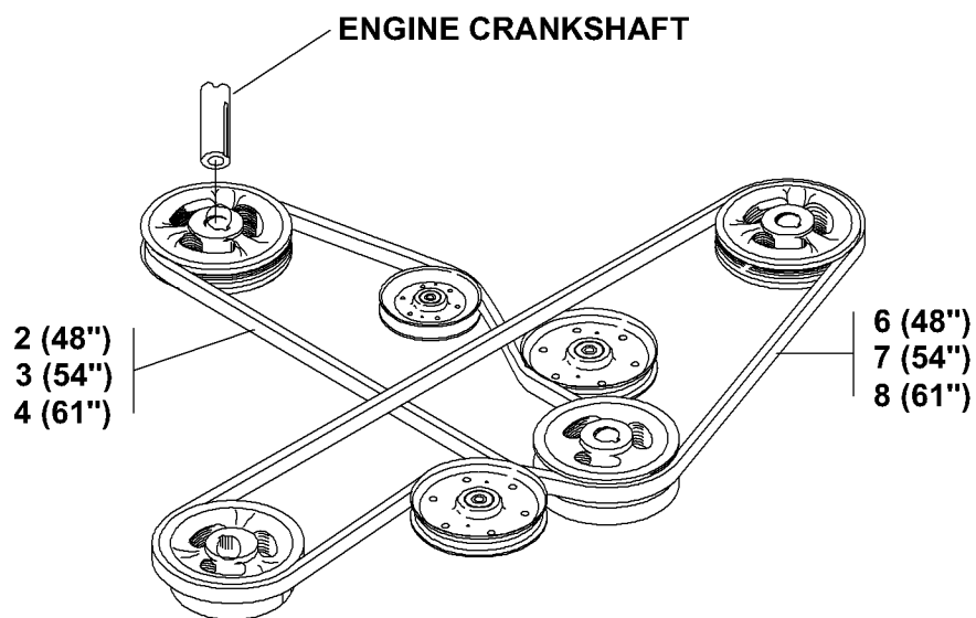
48", 54" & 61" LAYOUT
