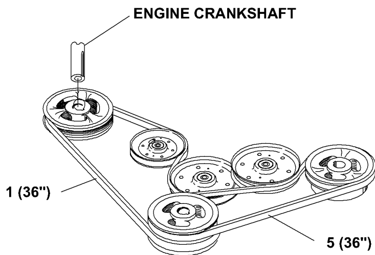
36" LAYOUT
