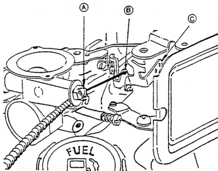
Figure 6. THROTTLE CONNECTION MODEL 6002 & 6032
