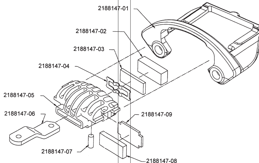
BRAKE ASSEMBLY BREAKDOWN
