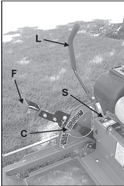
Lift and traction levers (operator's right side)
