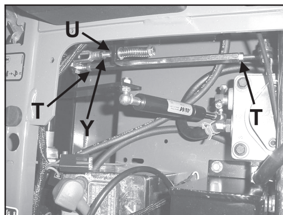
Right side adjustments (wiring harness removed for clarity)
