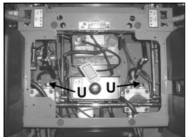
Compartment beneath the seat, viewed from above
