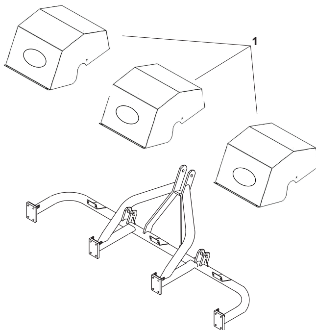
FIGURE 4 1. Guard Assemblies
