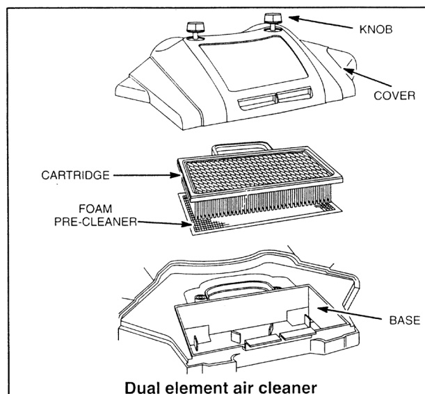
Dual element air cleaner
