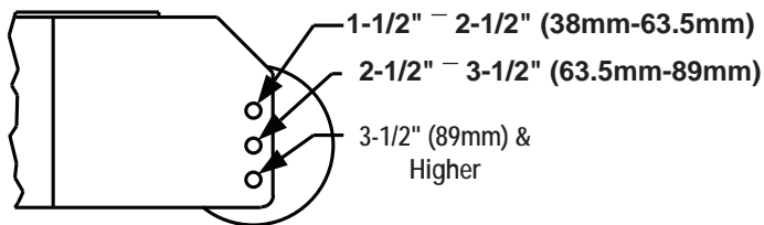
Height of cut ranges for roller adjustment
